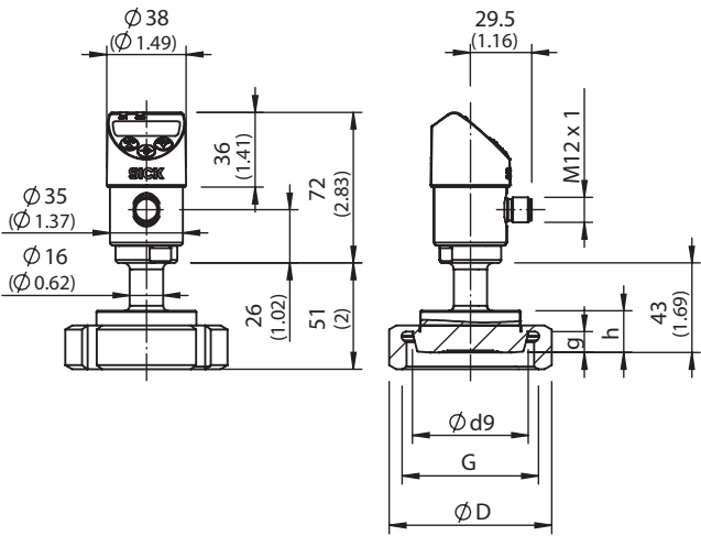
Dimensional drawing Conical coupling (DIN 11851) with union nut
