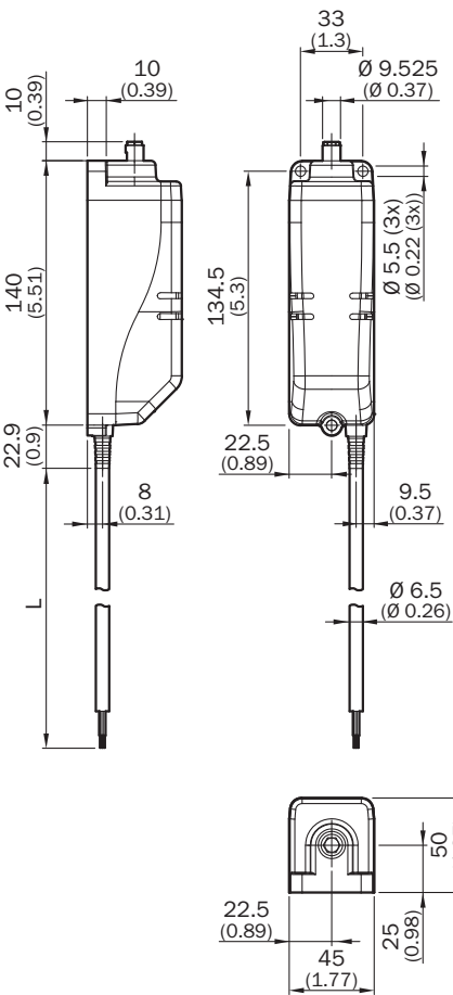
Dimensions in mm (inch)
