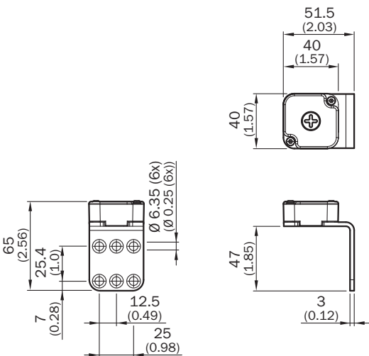
Dimensional drawing Actuator and mounting bracket
