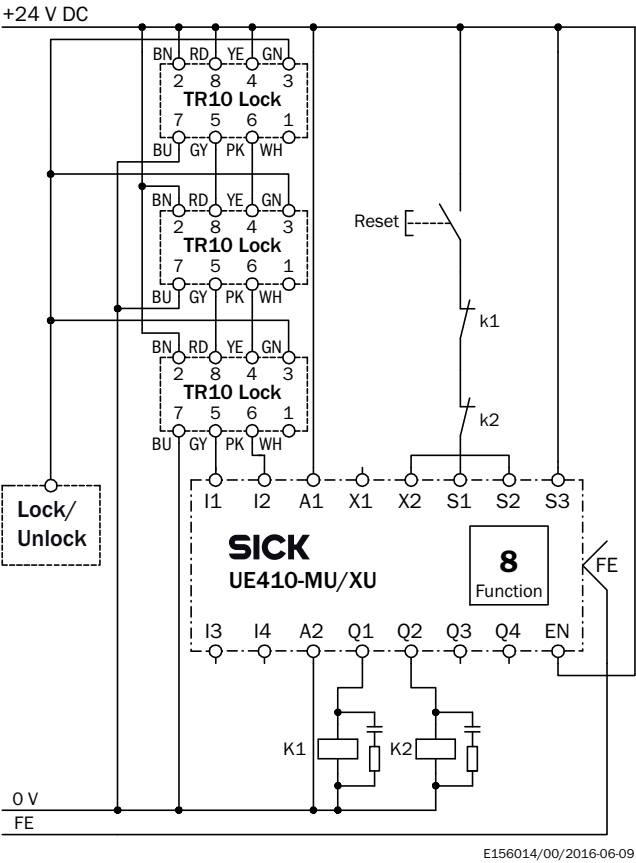
Connection diagram Series connection of three TR10 Lock safety locking devices to a Flexi Classic safety controller
