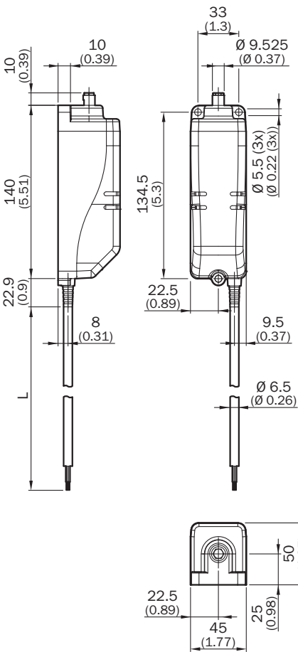
Dimensional drawing Sensor with cable
