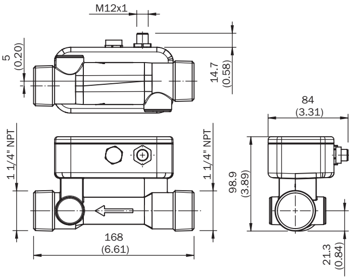
Dimensional drawing DN 25, 1 1/4" NPT
