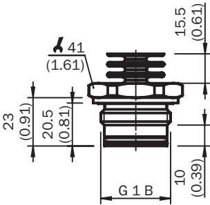
Dimensional drawing G 1 B with cooling section
