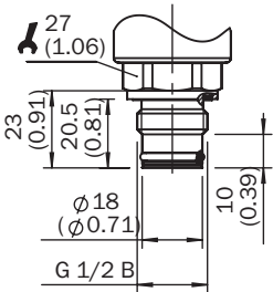
Dimensional drawing G ½ B flush mounted
