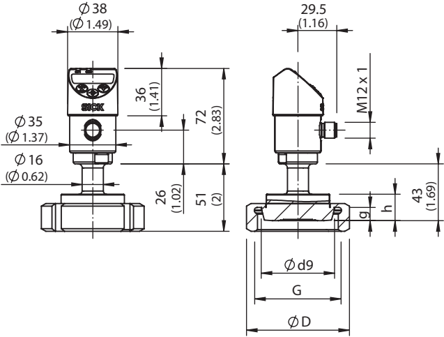
Dimensional drawing Conical coupling (DIN 11851) with union nut
