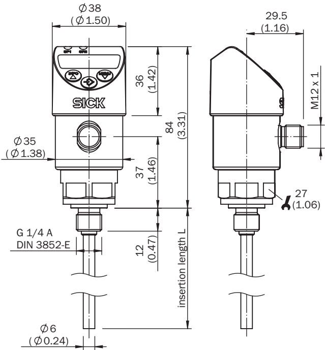
Dimensional drawing TBS with connection G 1/4 A according to DIN 3852-E
