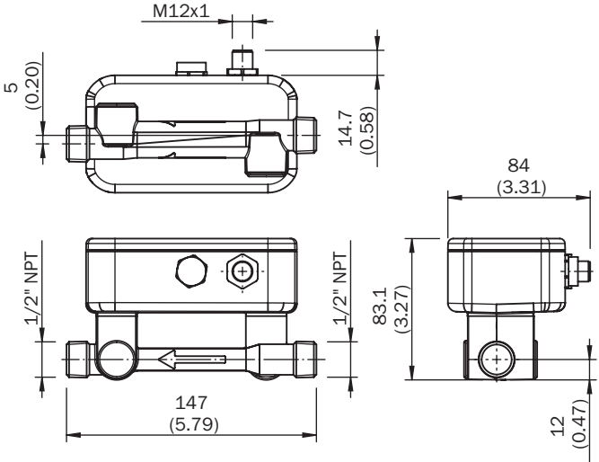
Dimensional drawing DN 10, 1/2" NPT
