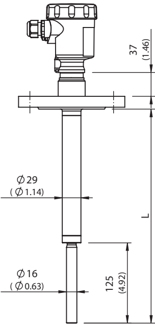
Dimensional drawing LBV331 flange
