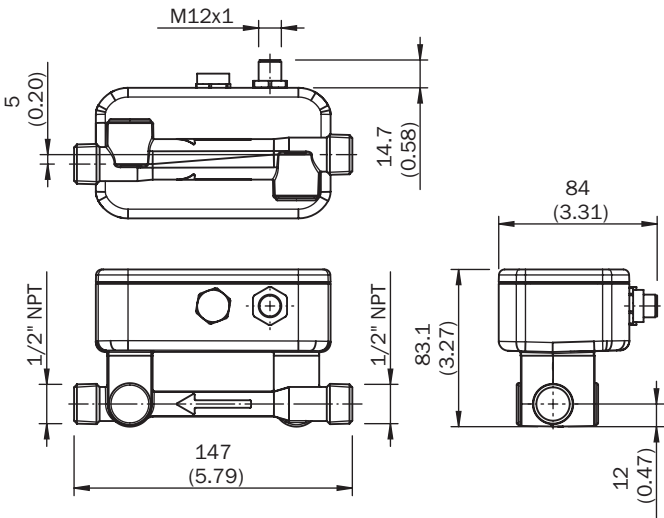
Dimensional drawing DN 10, 1/2" NPT
