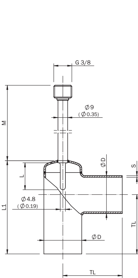
Protection tube with process connenection
