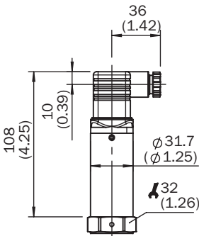
Dimensions in mm (inch)
