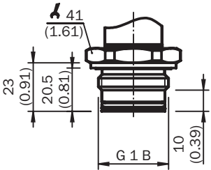
Dimensional drawing G 1 B without cooling section
