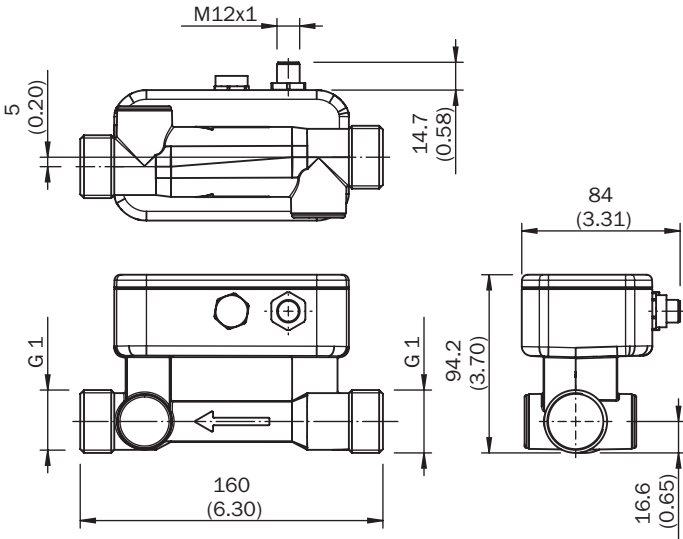
Dimensional drawing DN 20, G 1
