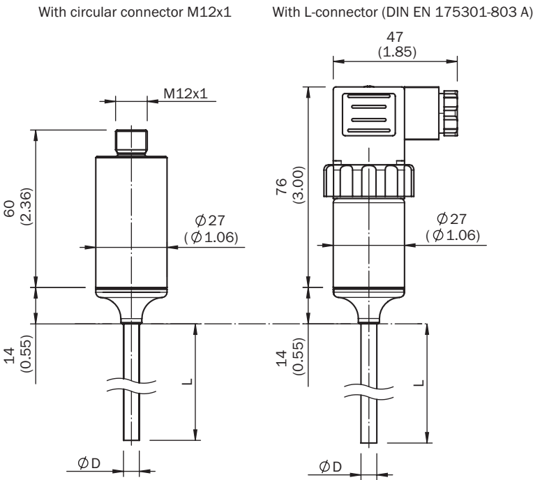
Dimensions in mm (inch) TCT-1
