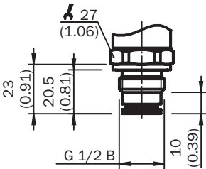
Dimensional drawing G <b>1/2</b> B without cooling section
