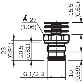
Dimensional drawing G <b>1/2</b> B with cooling section
