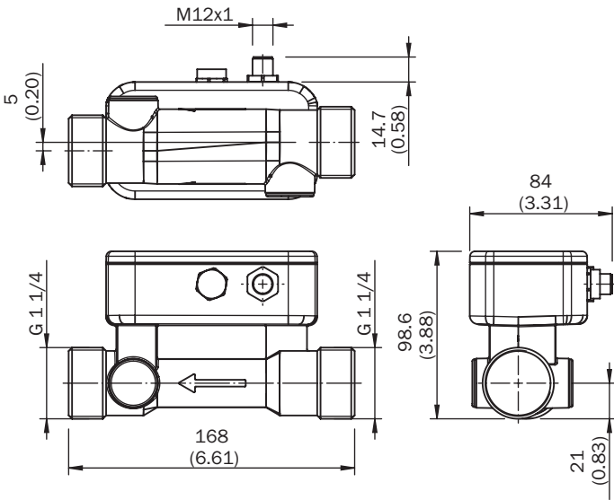
Dimensional drawing DN 25, G 1 1/4
