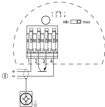
Connection diagram Transistor connection diagram
