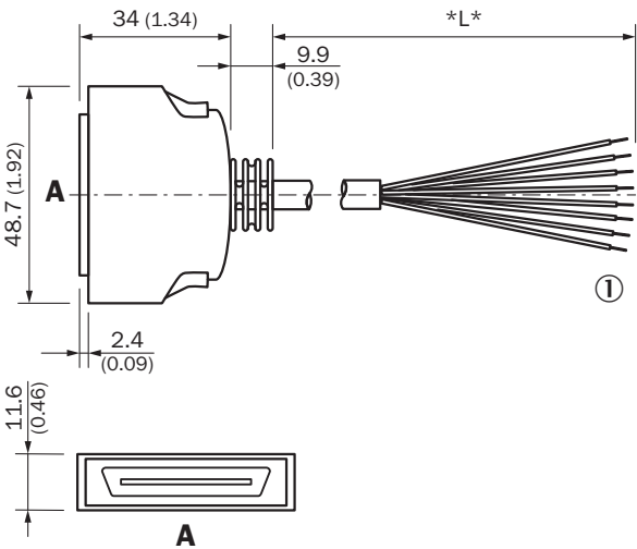
Dimensional drawing IO-EXP-AOD5
