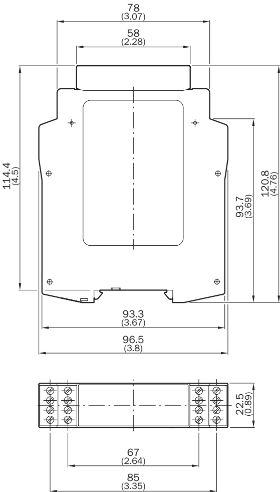
Dimensional drawing Flexi Classic main module
