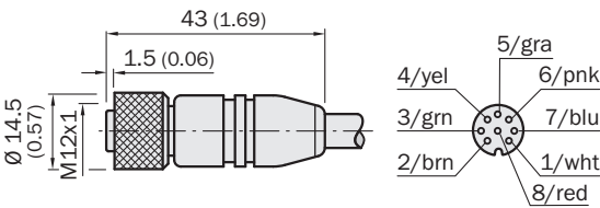
Dimensions in mm (inch)
