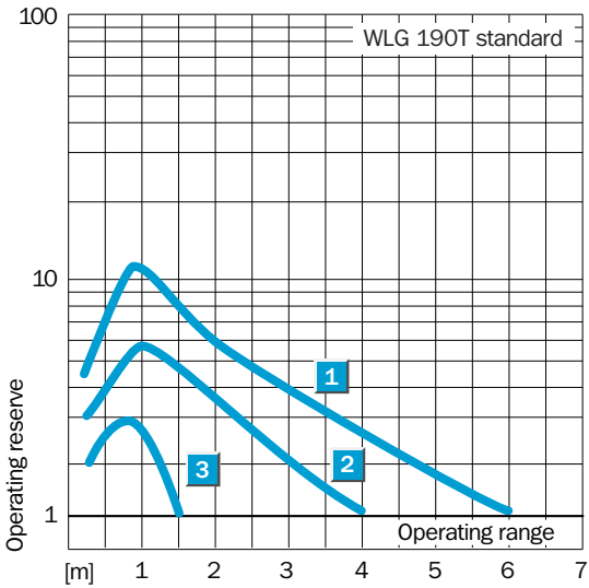
Characteristic curve WLG190T, 5.5 m
