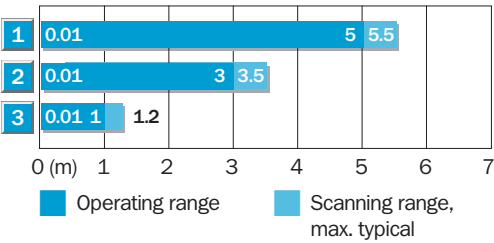
Sensing range diagram WLG190T, 5.5 m
