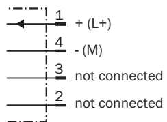
Connection diagram Cd-015
