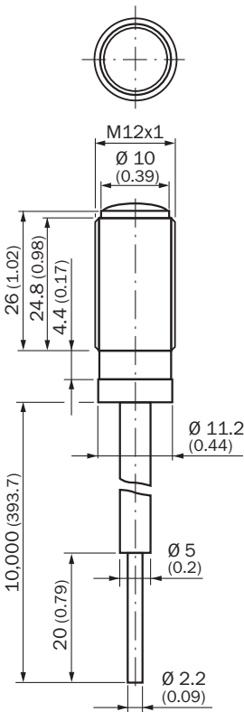
Dimensional drawing LL3-TX02-10
