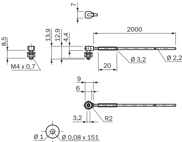
Dimensional drawing LL3-TR08
