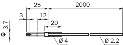
Dimensional drawing LL3-TG03, LL3-TV08
