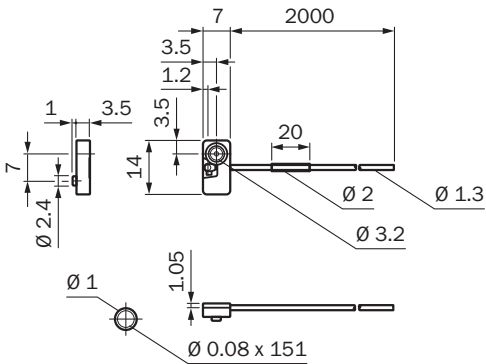
Dimensional drawing LL3-TE03
