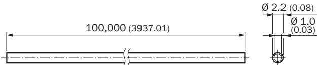
Dimensions in mm (inch)
