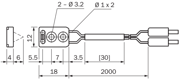
Dimensional drawing LL3-DC38
