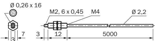
Dimensions in mm (inch)
