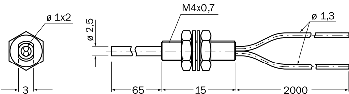
Dimensional drawing
