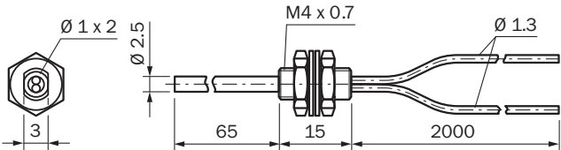
Dimensional drawing LL3-DK63Z
