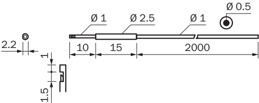
Dimensional drawing LL3-TV02
