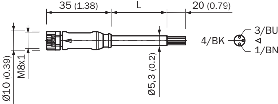
Dimensions in mm (inch)
