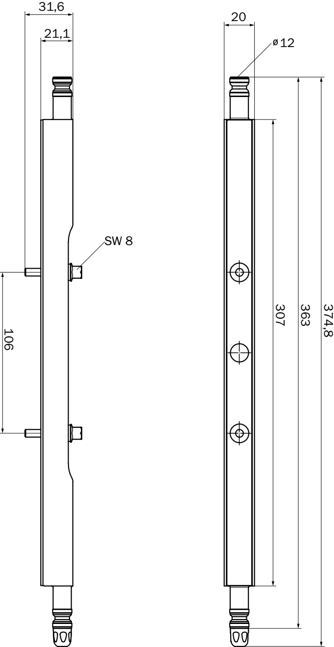
Dimensions in mm (inch)
