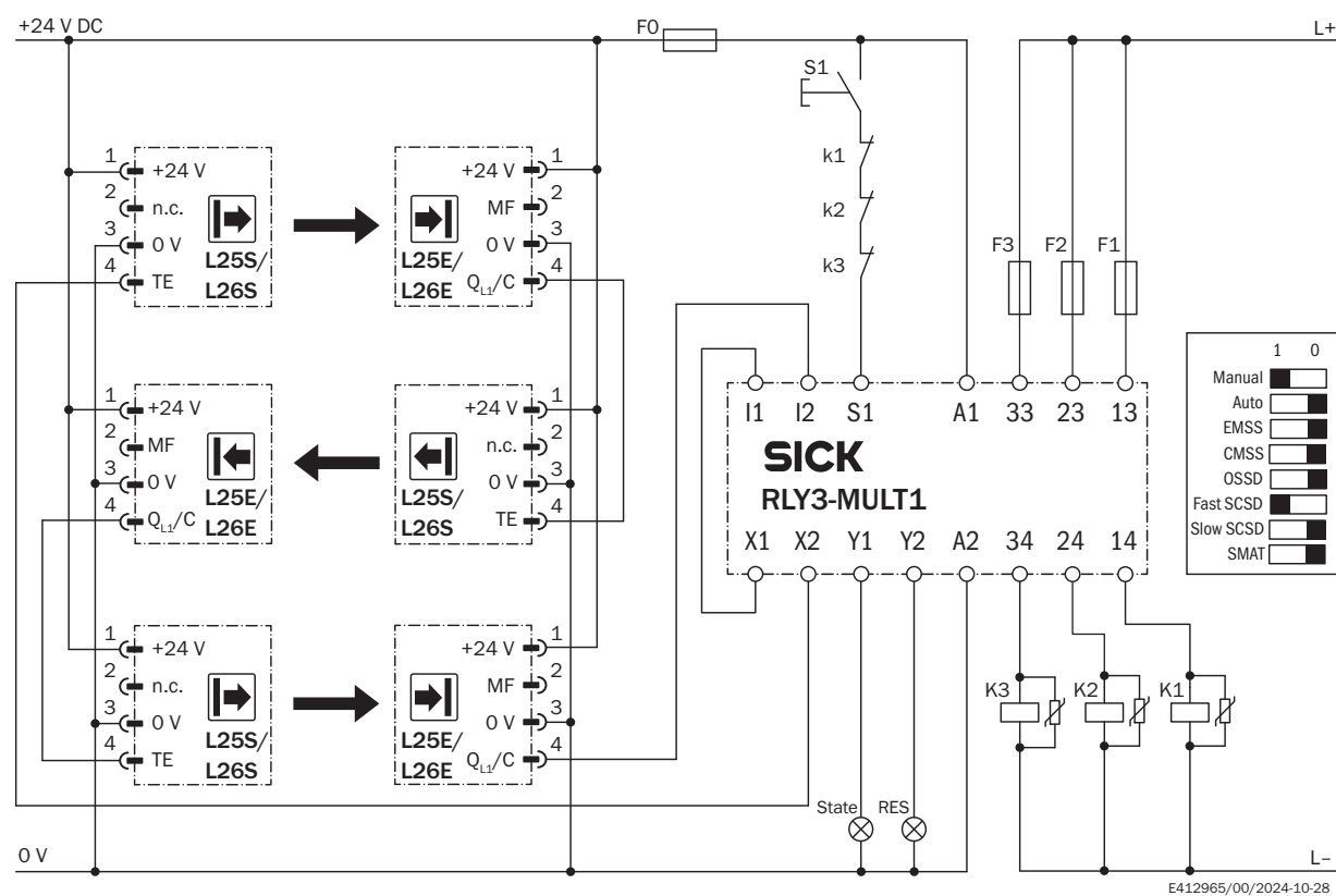
Connection diagram 3 x L25/L26 to RLY3-MULT1, with restart interlock and external device monitoring
