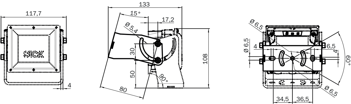
Dimensions in mm (inch)
