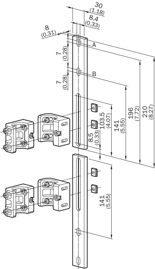
Dimensions in mm (inch)
