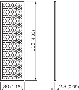
Dimensions in mm (inch)
