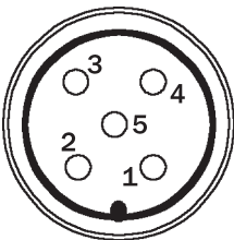
OUT/US (female contact)
