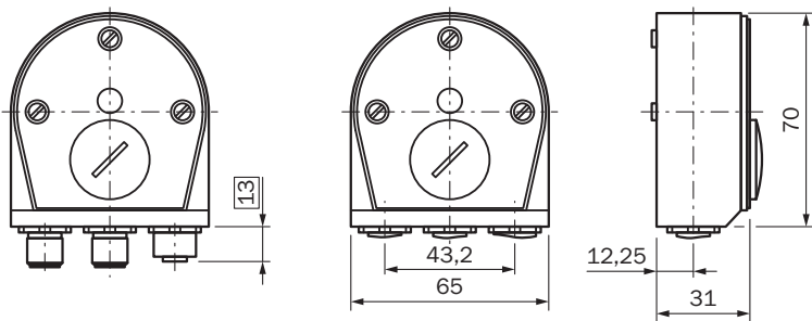
Dimensions in mm (inch)
