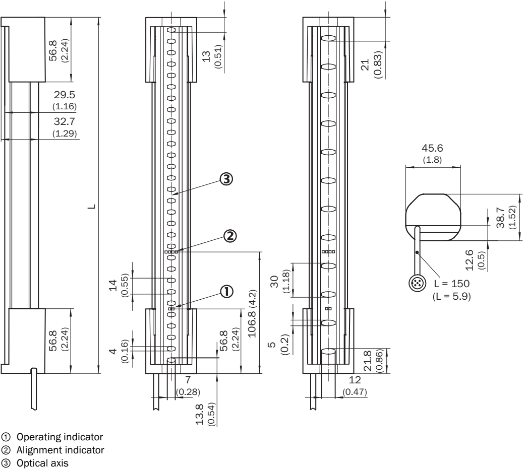
Dimensional drawing (Dimensions in mm (inch))
