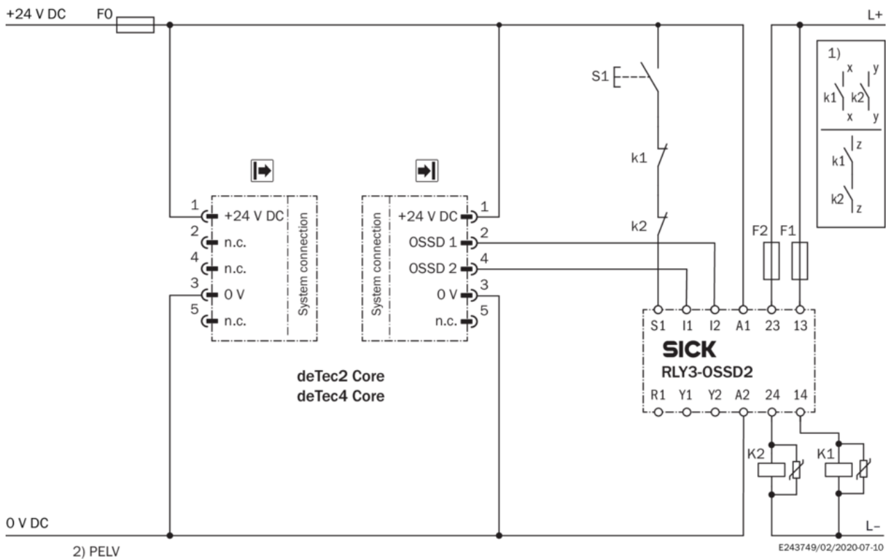
Connection diagram deTec2 Core safety light curtain to RLY3-OSSD2 safety relay
