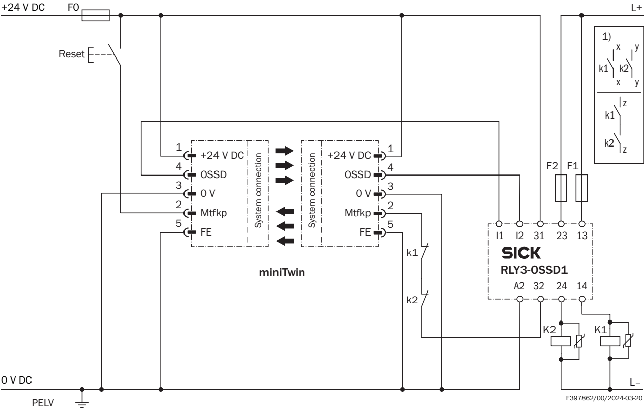
Connection diagram miniTwin safety light curtain to RLY3-OSSD1 safety relay with restart interlock and external device monitoring
