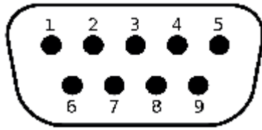
D-Sub 9P Male Pinout
