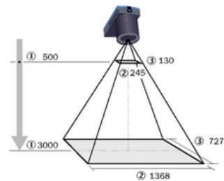
Figure 29: Field of view V2D8509R-xxxxxxxxx, focal length: 25 mm
