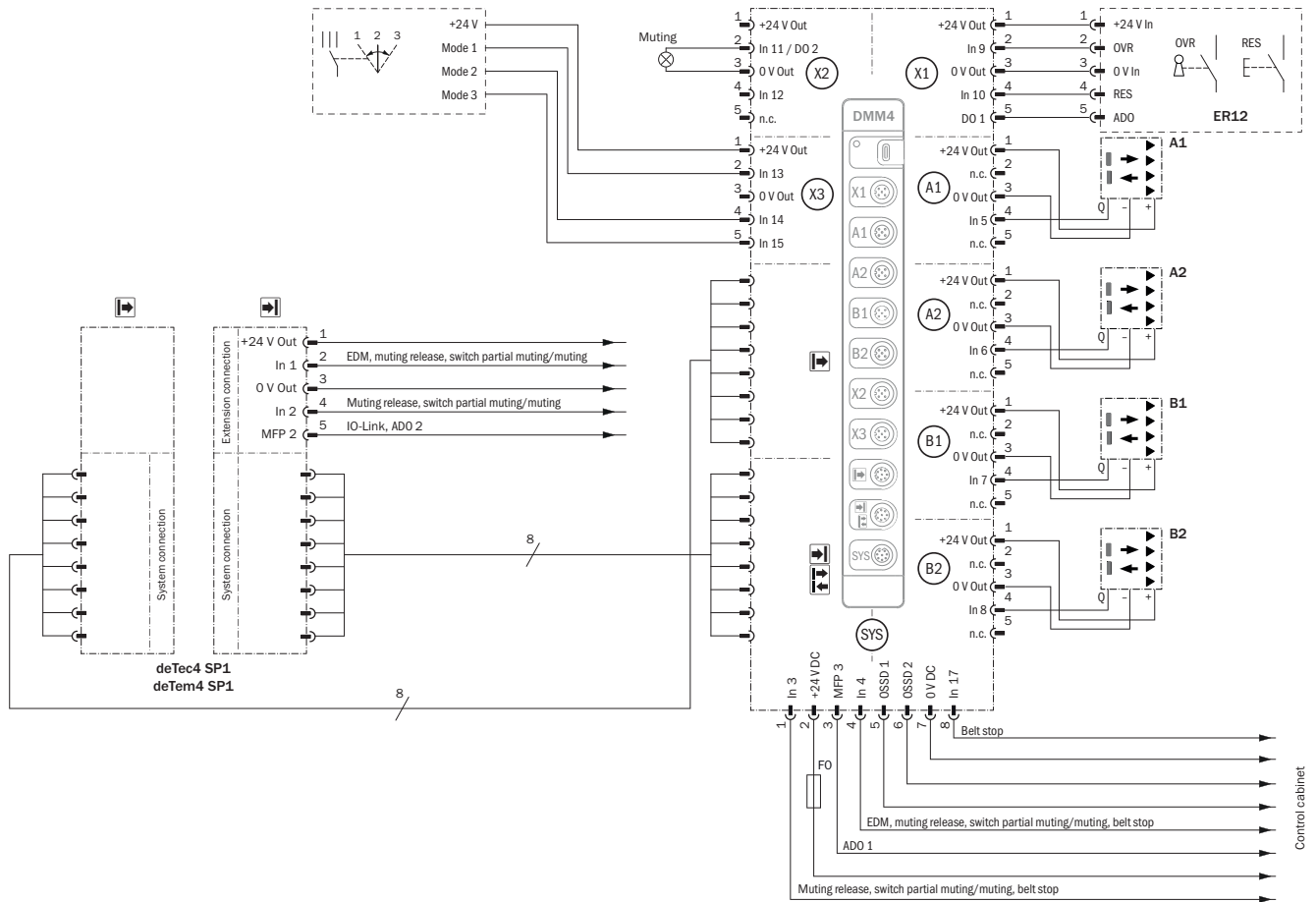
Connection diagram deTec4 / deTem4 on DMM4, muting, reset, override, operating mode selection
