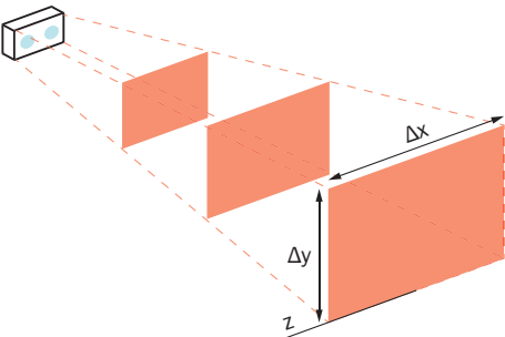
Functional principle Detection volumes and 2D measuring ranges
