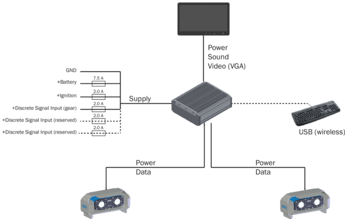
Connection diagram Visionary-B CV, kit B
