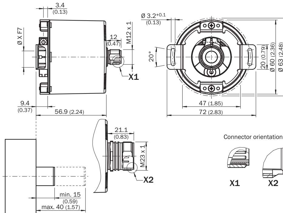
Dimensional drawing Blind hollow shaft, axial male connector M12 and M23
