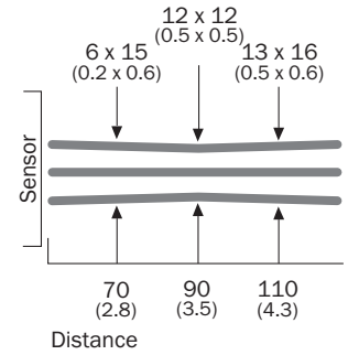
Sensing distance 90 mm
